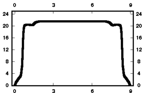
FIG. 9. At \beta=10 , energy along the path (as a function of u ) for the 2D vacancy problem.
