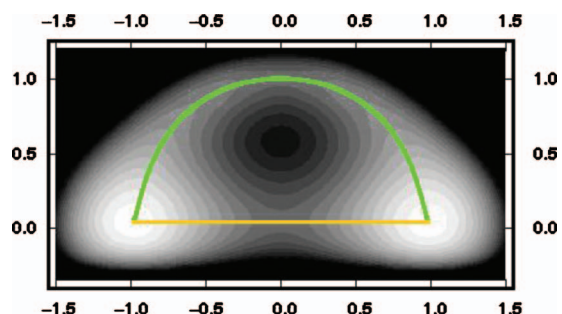
FIG. 2. A contour plot of the 2D potential; see Eq. (8). The two possible transition paths from one minimum to the other are indicated in the figure. The straight yellow line corresponds to the direct route; the green arc denotes the circular route. Along either path the barrier energies are the same.
