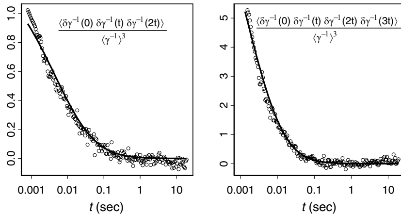
FIG. 3. Three-time and four-time correlation functions of fluorescence lifetime fluctuation of the same Fre molecule as in Fig. 2, which agree well with the predictions from the GLE with FGN (solid lines according to Eq. (13) and (14) respectively) using the same parameters obtained from the data fitting in Fig. 2.
