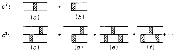
Figure 4. Diagrams for Q(\alpha, t) expressed in terms of the t matrices. The first row is proportional to c^2 , and the second to c^3 .
