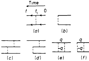
Figure 1. Diagrams for Q(\alpha, t) .
