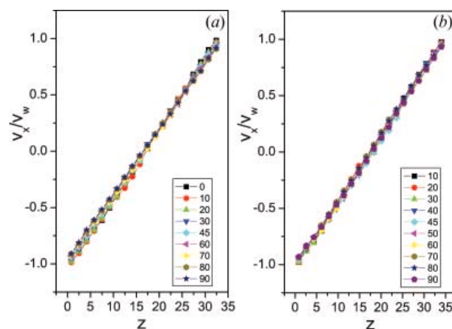
Figure 2. Scaled tangential velocity v_x/V_w plotted as a function of z : (a) in the XZ configurations, with the corresponding values of \theta_B listed in the inset; (b) in the XY configurations, with the corresponding values of \phi_B listed in the inset.
