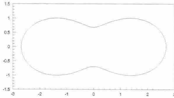
Figure 1. The curve \Gamma used in example 1.
