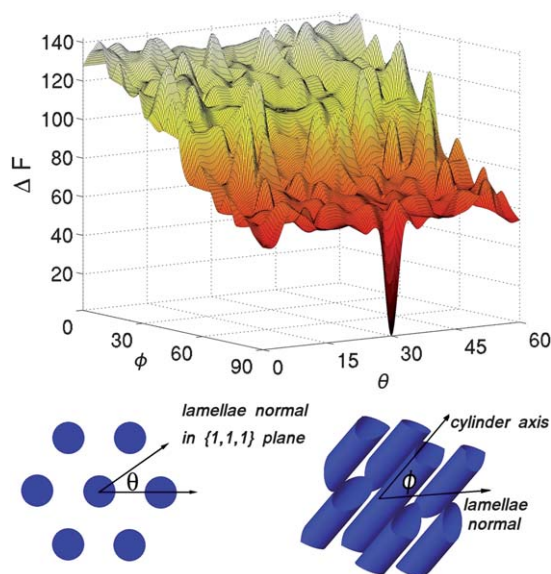
Fig. 1 Plot of the C \rightarrow L nucleation barrier as a function of the L-orientation. The parameters are f_A = 0.45 and \chi N = 11.4 . Because of the symmetry of the L and C phases, the surface is drawn in region 0^\circ \leq \phi \leq 90^\circ , 0^\circ \leq \theta \leq 60^\circ , where \phi and \theta are defined in the lower part of the figure.
