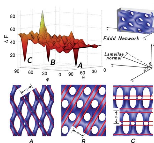
Fig. 3 Fddd \rightarrow L nucleation barrier in terms of L's orientations. The orientation is described by \theta and \phi , which are defined in the upper right part of the figure. The barriers are calculated at \chi N = 12.0 and f_A = 0.45 . Only the regions 0^\circ \leq \phi \leq 90^\circ and 0^\circ \leq \theta \leq 90^\circ are shown because of the symmetry.
