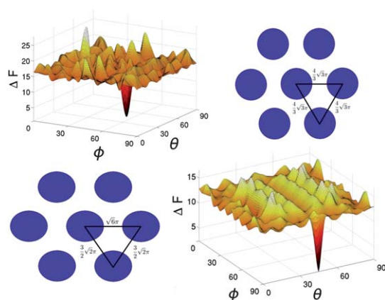
Fig. 2 G \rightarrow regular C (upper) and G \rightarrow distorted C (lower) nucleation barrier in terms of C's orientations. \theta and \phi are polar coordinate parameters for cylinder axis, and the rotation dimension of cylinders is not shown. The barriers are calculated at \chi N = 11.25 and f_A = 0.44 . Distances in the sketches of cylinders are in unit of q_0^{-1} .
